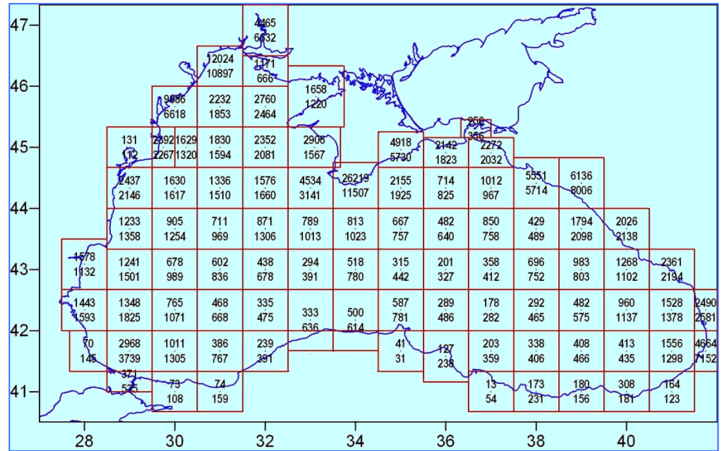
Distribution of oceanographic stations on squares in the Black Sea: lower –All-Russian Research Institute of Hydrometeorological Information – World Data Center upper –Marine Hydrophysical Institute RAS
