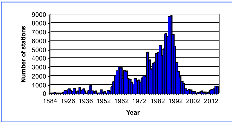
All-Russian Research Institute of Hydrometeorological Information – World Data Center Distribution of oceanographic stations on years
