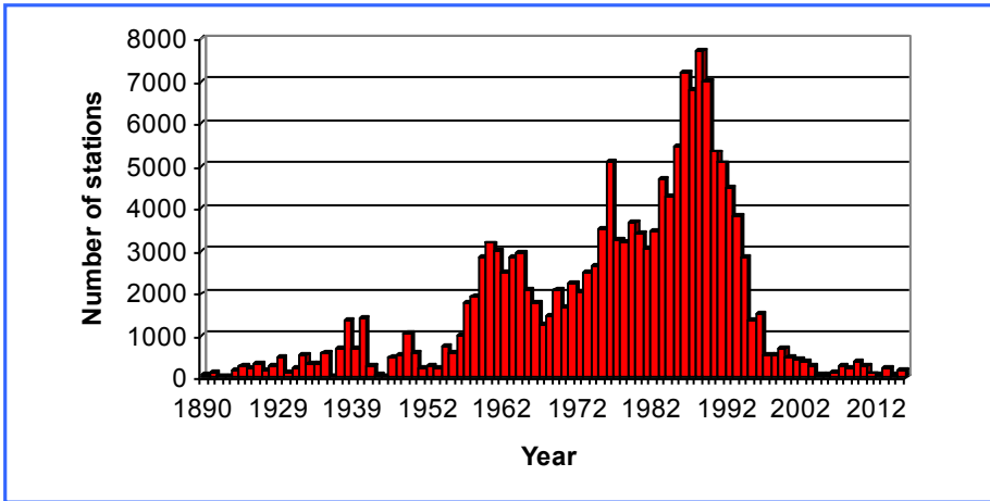
Marine Hydrophysical Institute RAS, Distribution of oceanographic stations on years
